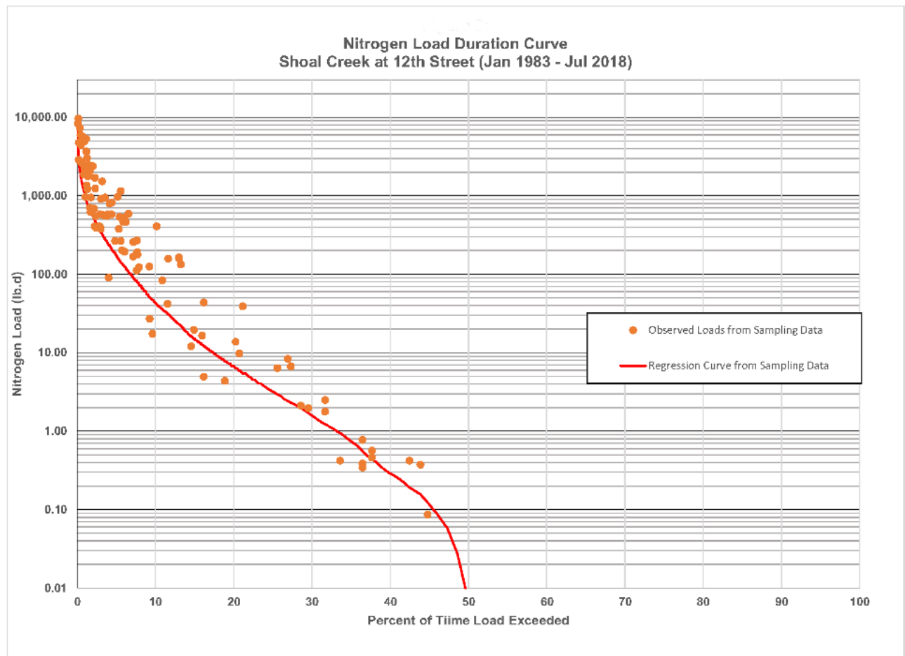
Figure 7 - Nitrogen Load Duration Curve
